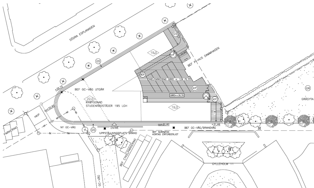
Situationsplan
